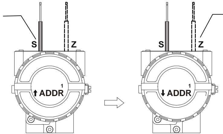
Figure 3.38 - Step 6 – LD293
