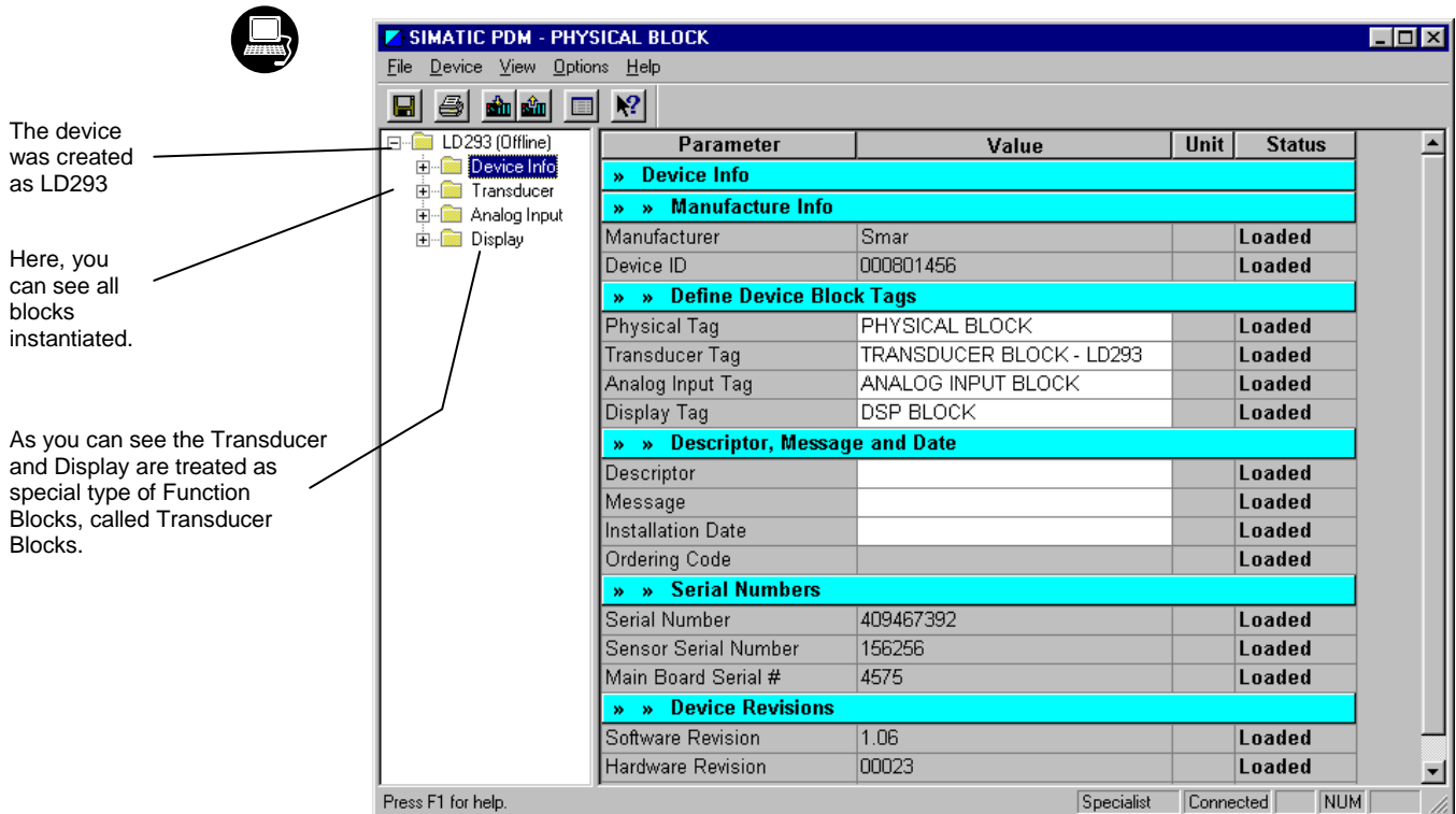
Figure 3.3 – Function and Transducers Blocks
