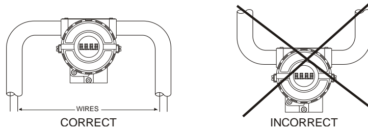
Figure 1.6 - Conduit Installation
