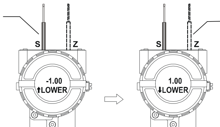
Figure 3.36 - Step 4 - LD293
