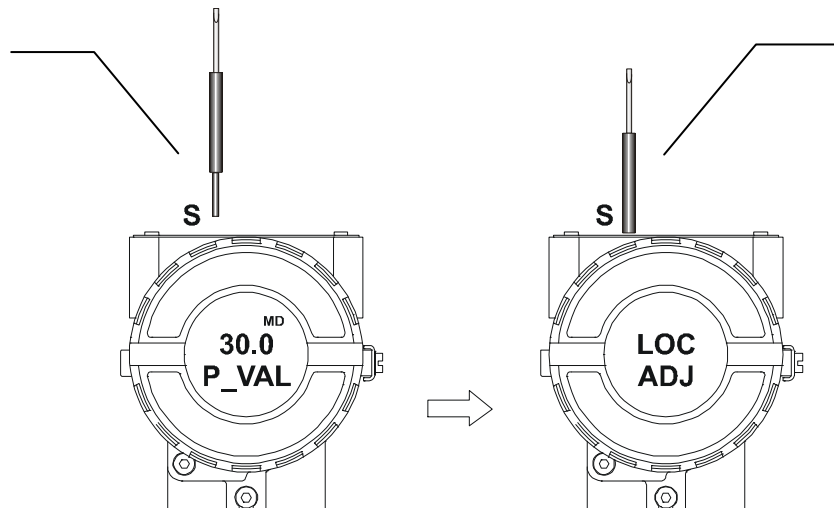
Figure 3.4 - Step - LD293
