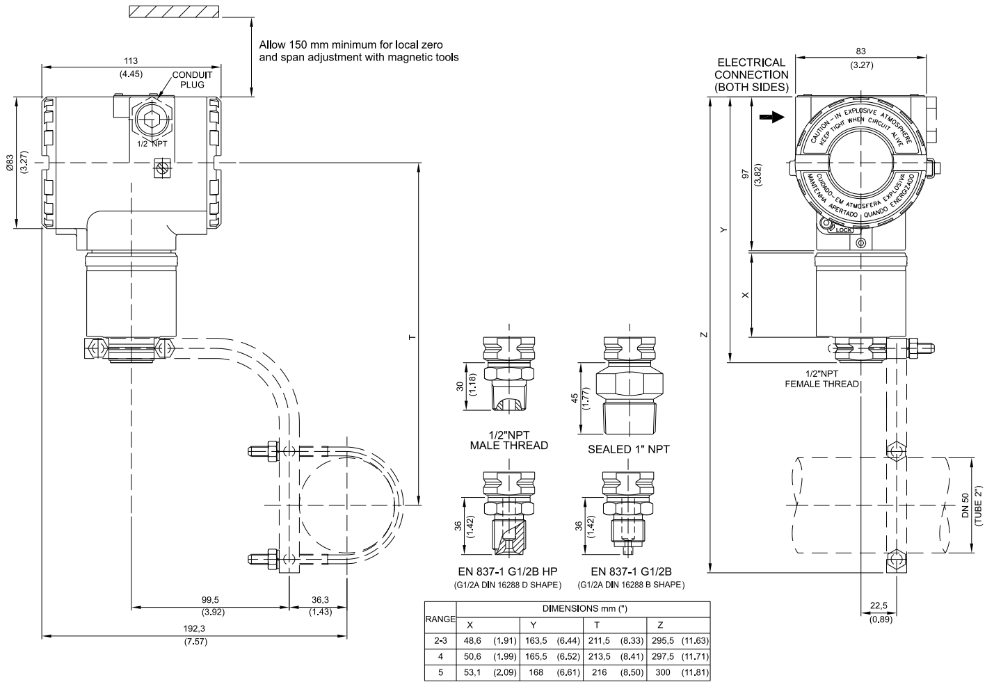
Figure 1.1 (a) - Dimensional Drawing and Mounting Position for LD293
