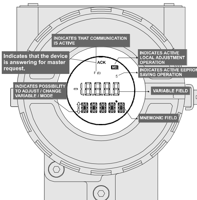
Figure 2.3 - LCD Display
