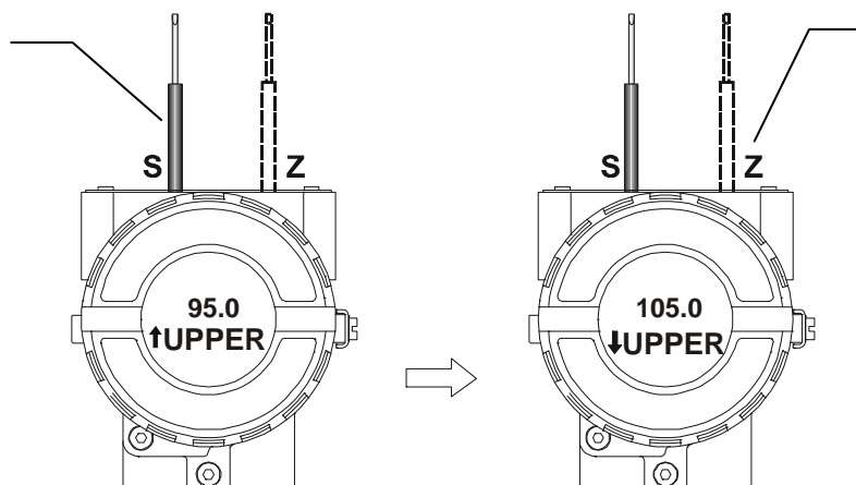
Figure 3.37 - Step 5 - LD293
