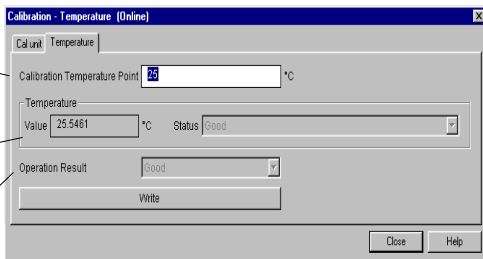
Figure 3.24 – The Temperature Trim Configuration Screen
