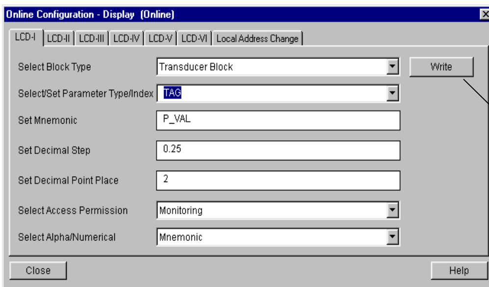
Figure 3.27 – Parameters for Local Adjustment Configuration
