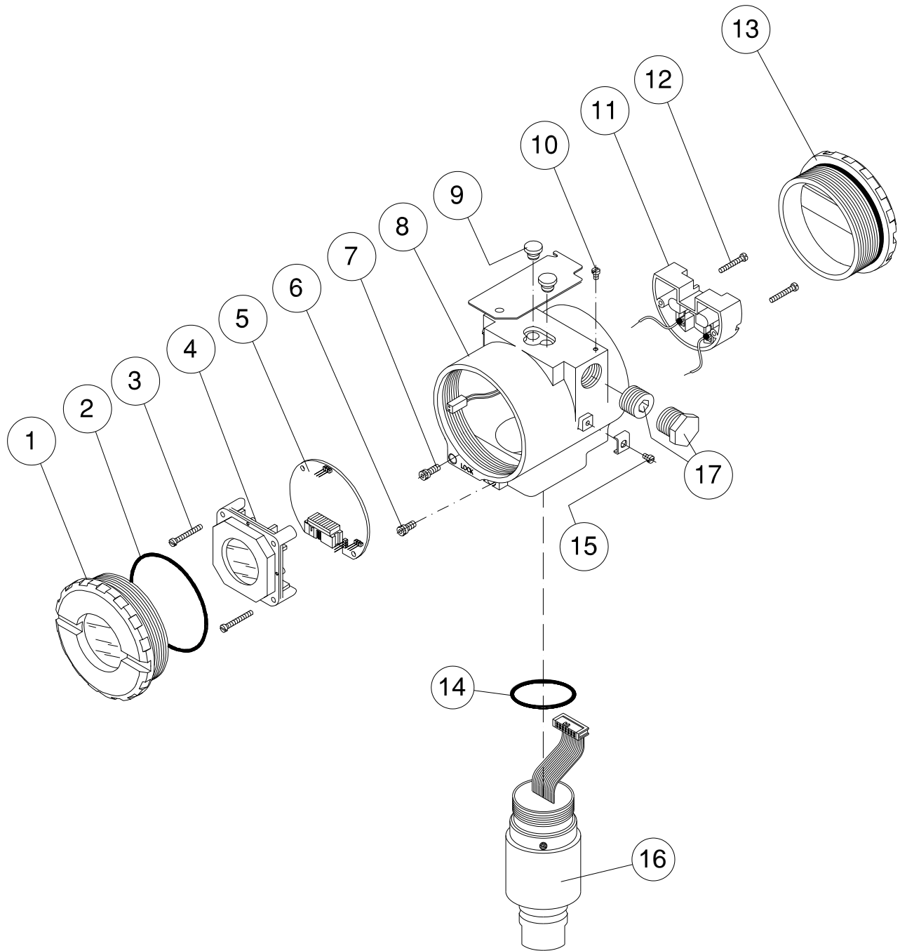
Figure 4.3 – Exploded View
