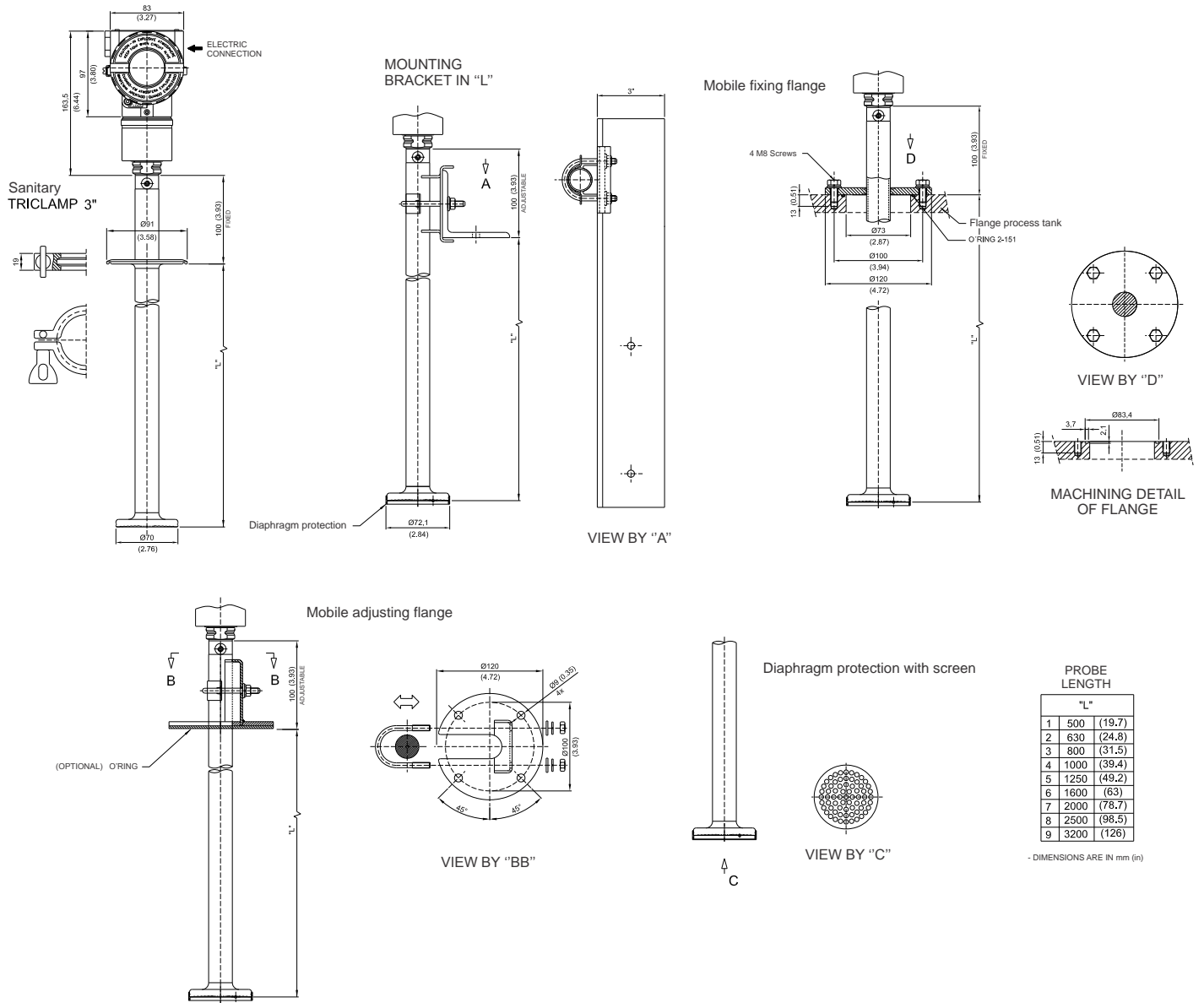
Figure 1.1 (e) - Dimensional Drawing and Mounting Position for LD293 – Level (Insertion)
