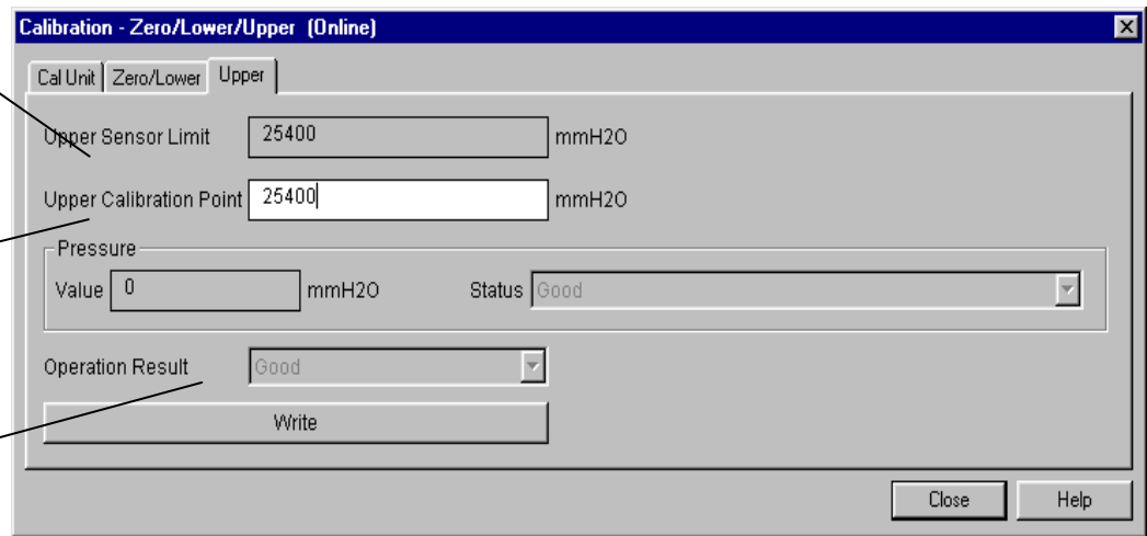
Figure 3.20 – LD293 Simatic PDM – Transducer Configuration Screen
